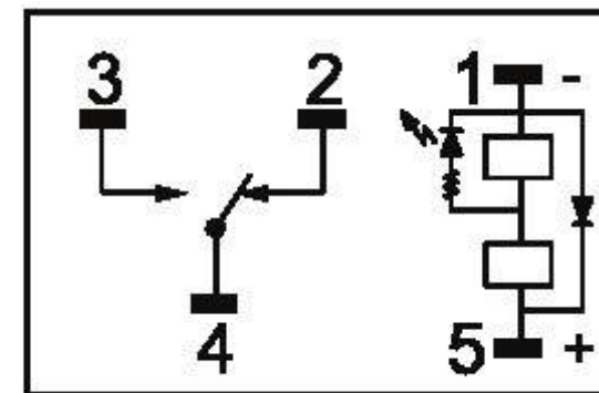
LED + Diode (DC)
