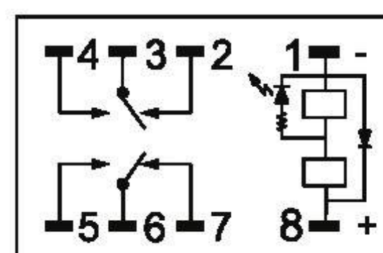
LED + Diode (DC)
